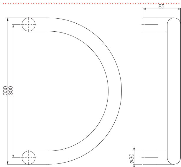
Back-to-back Inline Fix MPH573310
