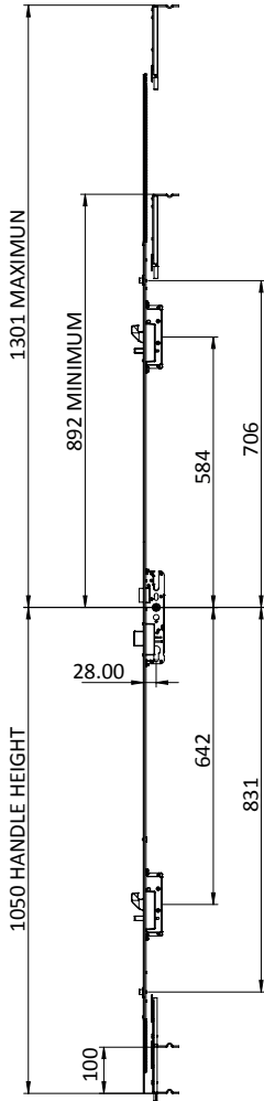
Single Door Lock YBF00128
