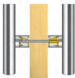
Back-to-Back Fixing
